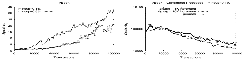
Figure 4. a) Incremental MFI Mining, and b) Itemsets Processed
