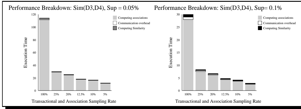
Fig. 2. Sampling Performance
