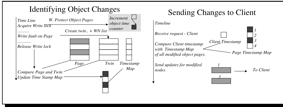
Figure 2. Efficient Shared Data Updates
