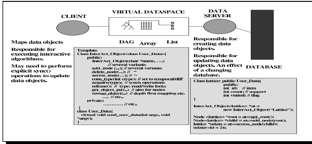
Figure 1. Interactive Client-Server Mining
