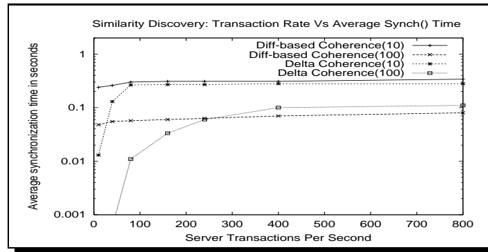
Figure 5. Effect of Transaction Rate on Similarity Performance
