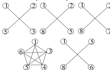
Figure 2. Equivalence Class and Uniform Hypergraph Clique Clustering
