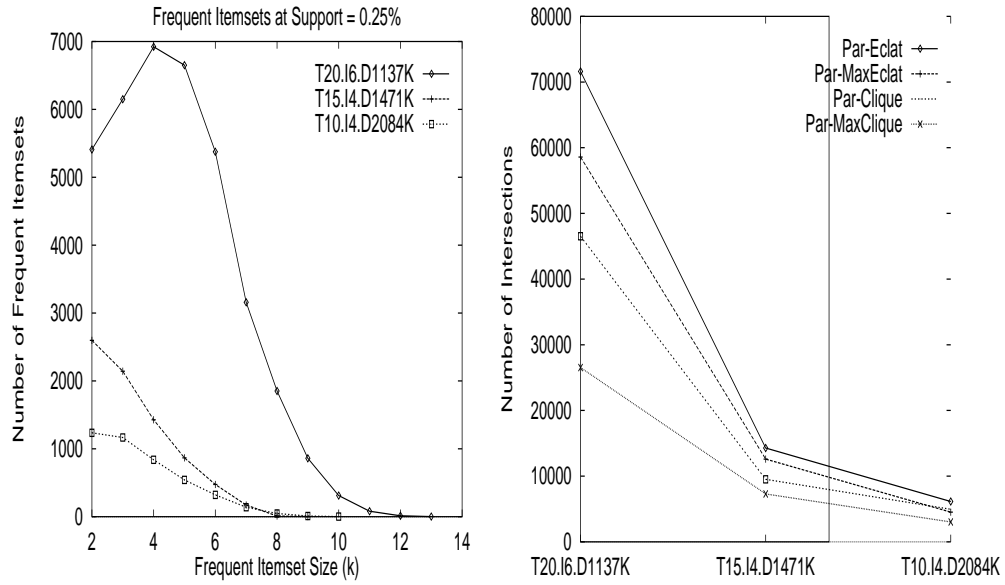
Figure 10. a) Number of Frequent k -Itemsets; b) Number of Intersections
