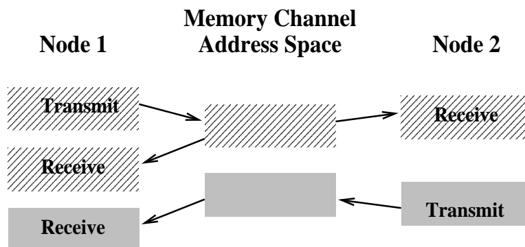
Figure 5. Memory Channel space. The lined region is mapped for both transmit and receive on node 1 and for receive on node 2. The gray region is mapped for receive on node 1 and for transmit on node 2.
